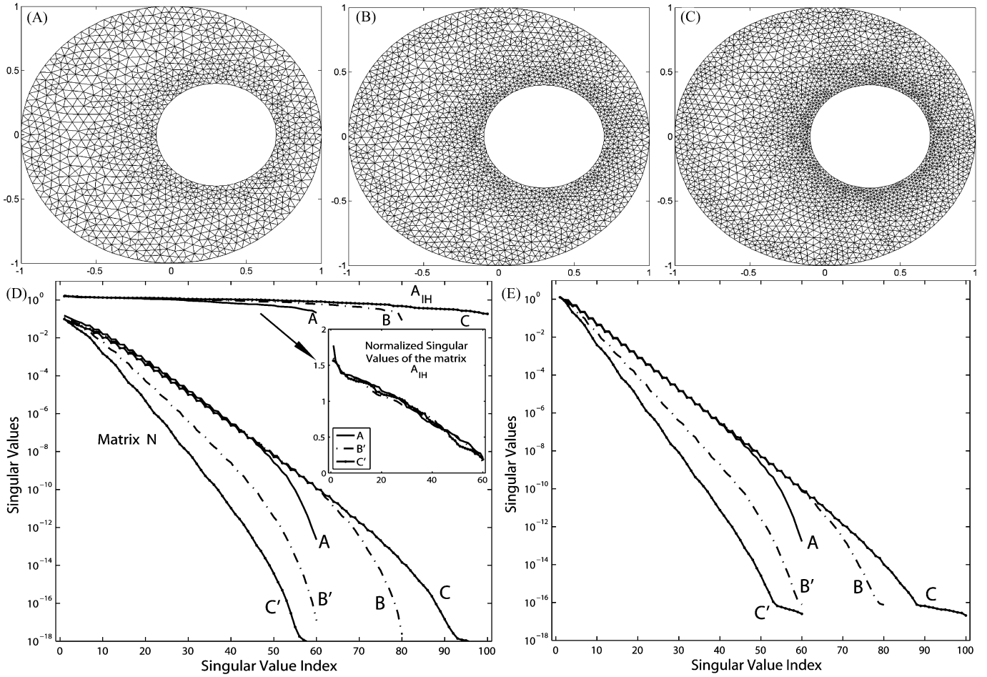
Fig. 2. Effects of uniform h -refinement on the transfer matrix K and its components. (A) Mesh with 60 nodes on heart. (B) Mesh with 80 nodes on heart. (C) Mesh with 100 nodes on heart. (D) Singular values of N and A_{IH} plotted against the original index (A, B, C) and the normalized index (A, B', C'). (E) Singular values of K plotted against the original index (A, B, C) and the normalized index (A, B', C').
