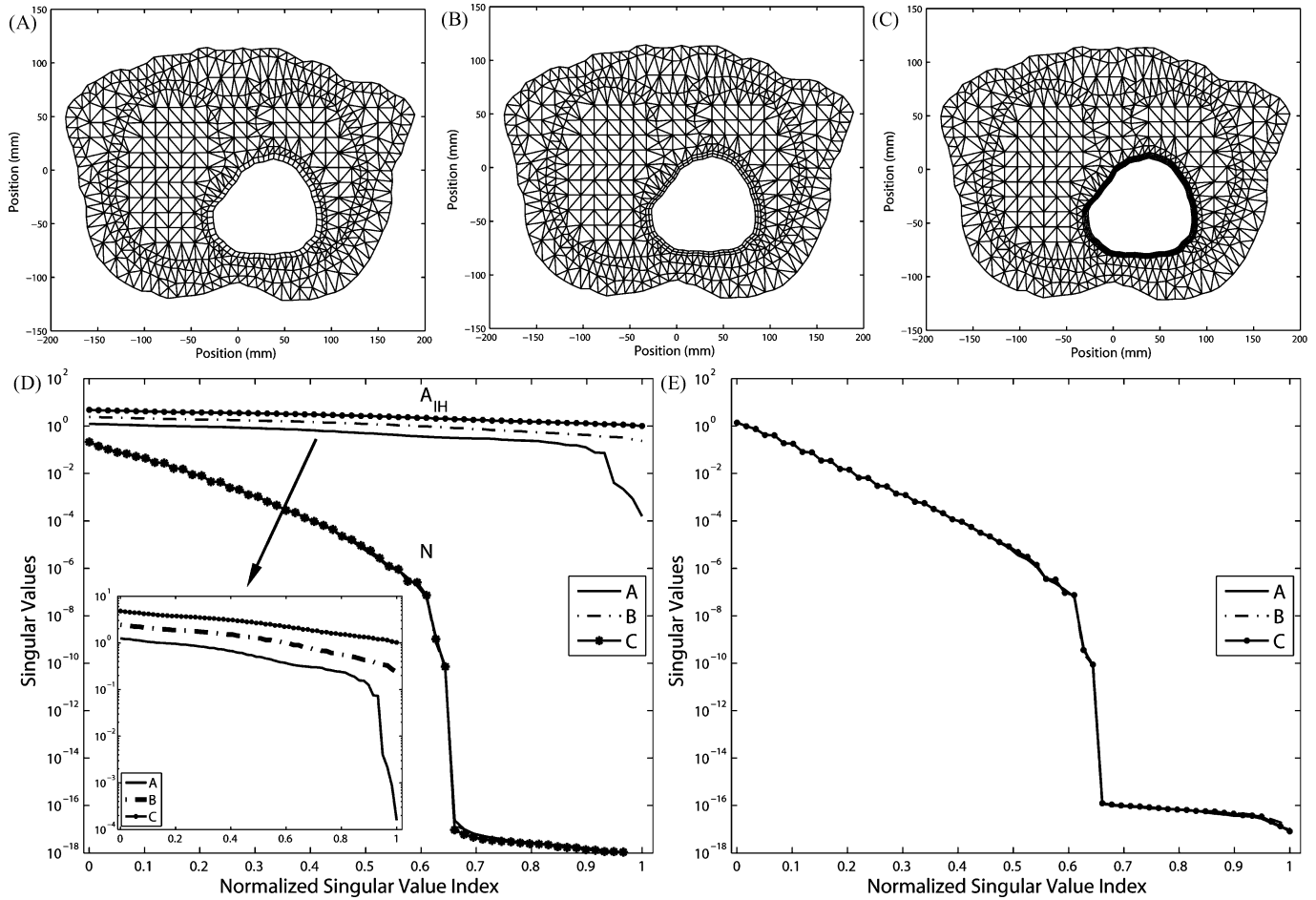
Fig. 12. Refining the resolution normal to the heart. (A) One layer of quadrilaterals around the heart. (B) Two layers of quadrilaterals. (C) Four layers of quadrilaterals. (D) Singular values of N and A_{IH} . (E) Singular values of K .
