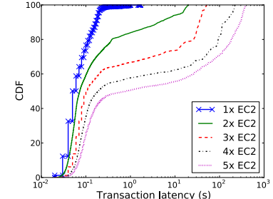
Figure 5: CDF of transaction latency (EC2 workload).
