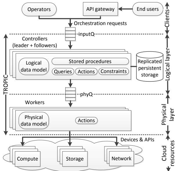
Figure 1: TROPIC architecture
