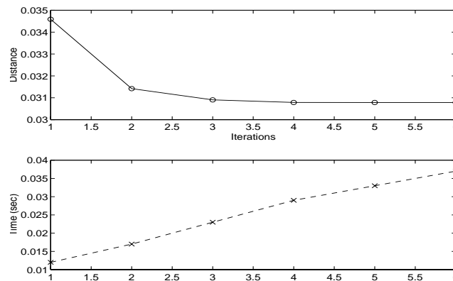
FIGURE 11. A. Minimum distance vs. iterations. B. Total time vs. number of iterations
